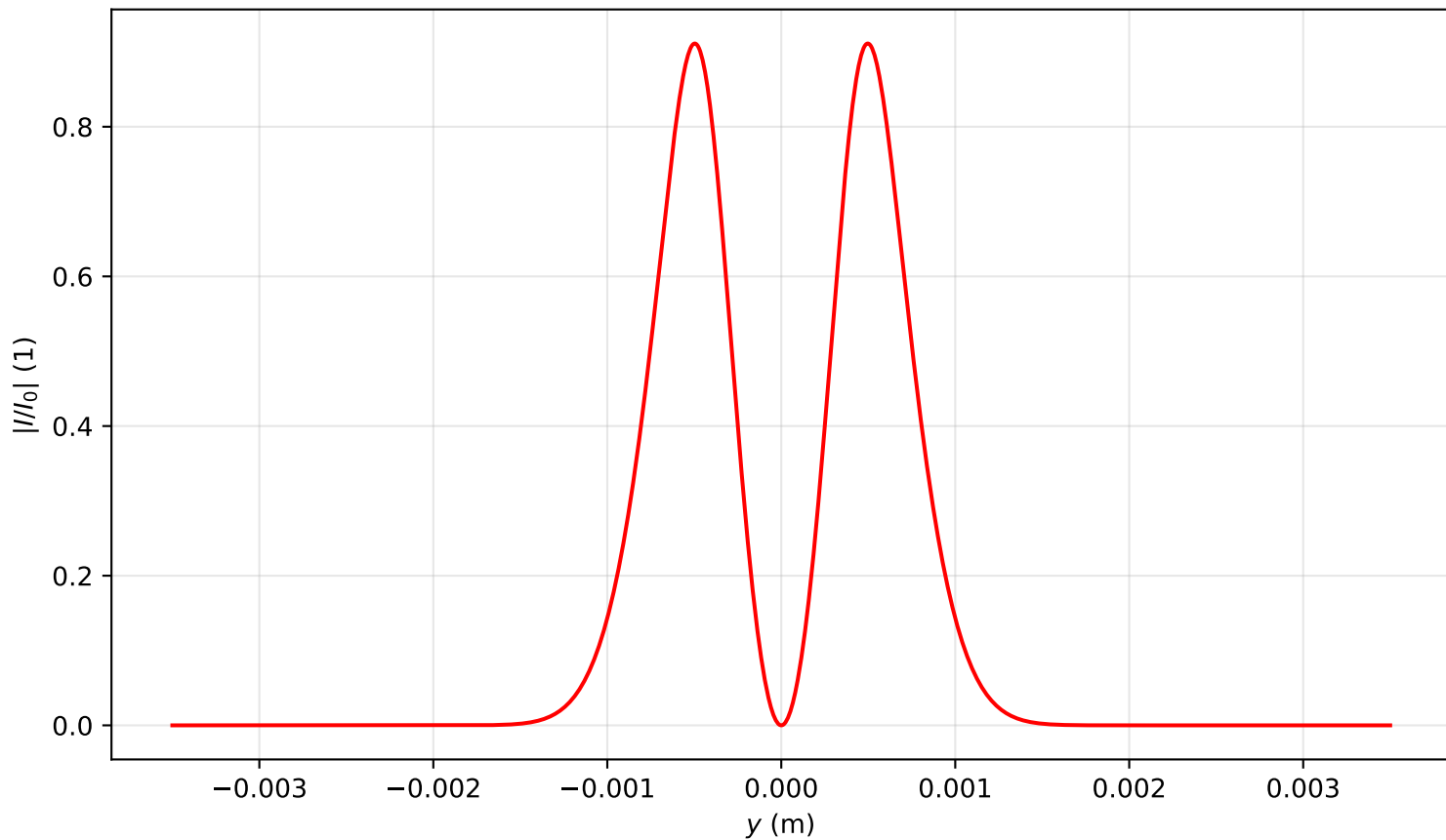
Intensity profile I(x=0, y, z=0.239)/I_0 , P_{in}=4.0P_{cr} , artificial time
